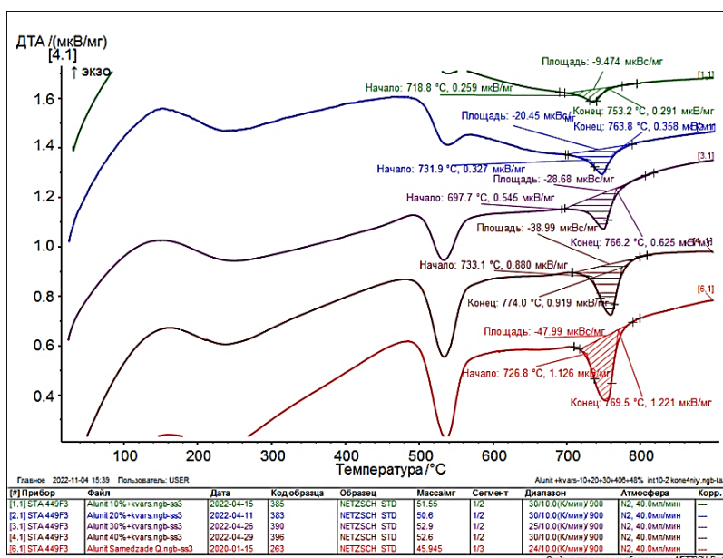
Fig. 2. Zones of endoeffect of desulphurization associated with sulphates, for samples containing 10,20,30,40, 48% of mass content of alunite in the rock, obtained on a derivatograph with a speed range of 10 k/min.
